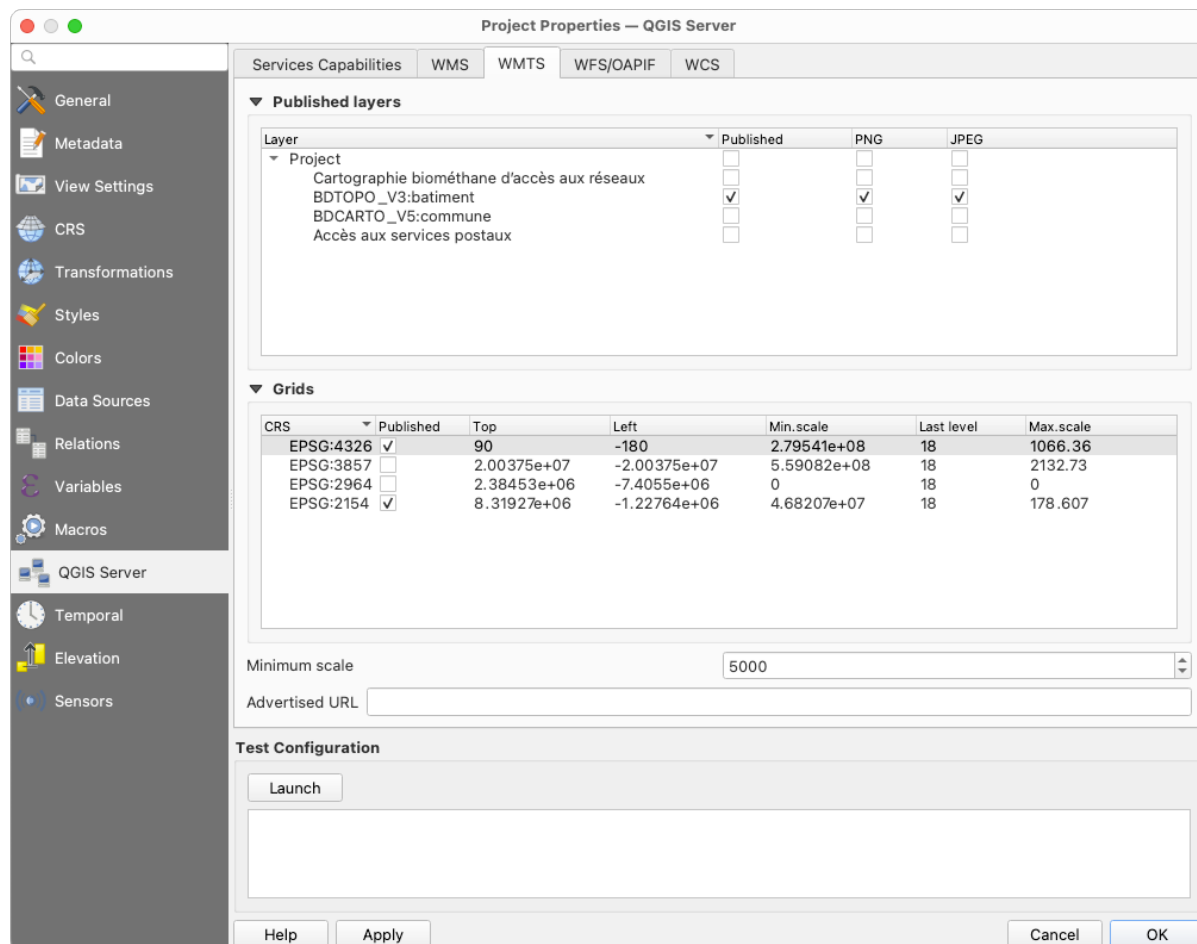
2.4 Fig. : Definitions in the WMTS tab
