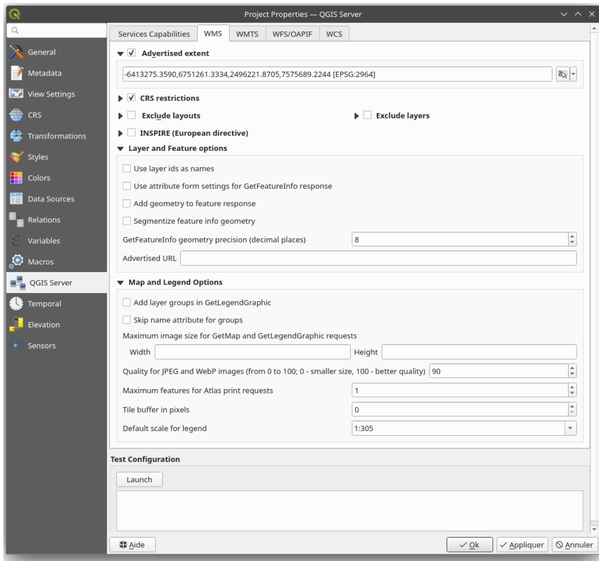
2.3 Fig. : Definitions in the WMS tab
