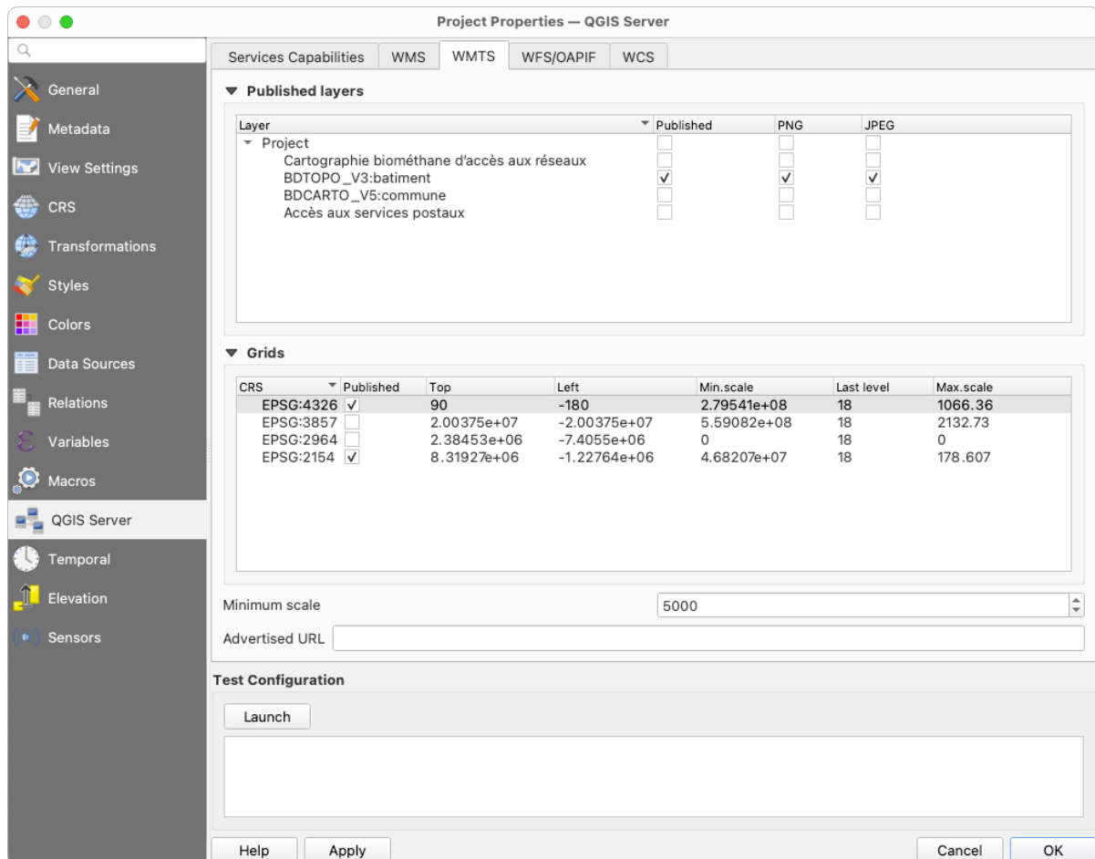
2.4. ábra: Definitions in the WMTS tab
