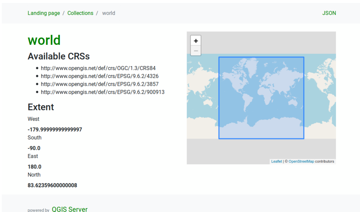
☒ 3.25: Server OAPIF collection detail page
